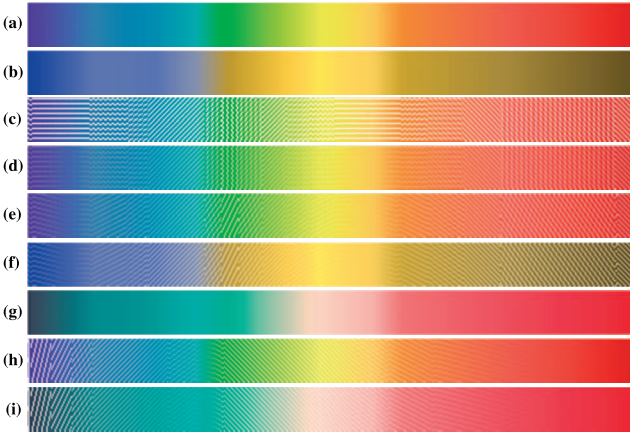
Fig. 6. (a) The colors in the visible spectrum from blue (shortest wavelength) to red(longest wavelength)— C_S . (b) The image as perceived by a deuteranope— C_P . (c) After overlaying the line-based patterns based on the distance from the deuteranope’s color plane— C_T . Completely vertical lines show the maximum tendency toward green and as the lines rotate in a clockwise direction the tendency toward red increases. Note how these lines disturb the perception of the blues and yellows though the deuteranope can perceive these colors correctly. (d) After the pattern contrast is modified based on the distance of the original color from the deuteranope’s color plane— C_F . Note that now the blues and yellows are devoid of patterns to provide a secondary cue to the deuteranope on the fidelity of his color perception. However, note that the small slanted line segments are not continuous and hence interpreting the direction is still hard. (e) After shifting the overlaid patterns to achieve continuity of the lines. Note that the use of continuous lines makes it easier to observe the orientation. (f) This is (e) as perceived by a deuteranope. (g) The visible spectrum as perceived by a Tritanope. (h) This is the pattern overlaid image generated by our method for the tritanope. (i) This is (h) as perceived by a tritanope.
