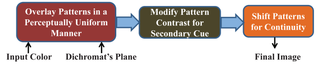
Fig. 5. Pipeline of our pattern augmentation method.
