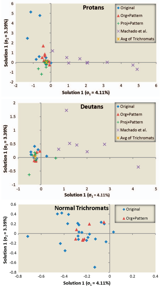
Fig. 13. Results of the user study based on both tasks and analyzed using dual scaling. Plot obtained after projecting the collected data onto the two dimensions (solutions) that best describe the relationships among the data. (Top) Results of the protan group for the various techniques, compared with the mean of the answers of the normal trichromats. (Middle) Results of the deutan group, also compared with the mean of the answers of the normal trichromats. (Bottom) Comparison of the answers of normal trichromats for the original images with and without enhancing with the patterns.
